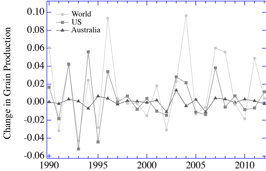
FIG. 2: Correlations of changes in grain production - Comparison of change in world (circles), US (squares) and Australian (triangles) grain production as a fraction of total world production by weight [6]. The correlation is small between world and Australia production changes (0.17), but high between world and US production changes (0.7).
