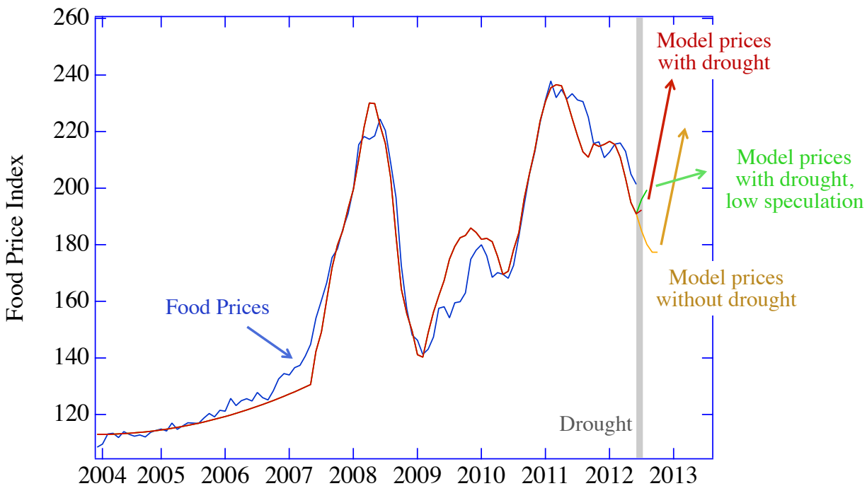
FIG. 1: Food prices and model simulations - The FAO Food Price Index (blue solid line) [19], the speculator and ethanol model [7], without the effects of the current drought (yellow line) with the effects of the current drought (red line), and with the effects of the drought, but with speculation reduced (green line). In all cases, corn-to-ethanol conversion is considered to be constant after Jan 2012 and stock prices and bond prices are considered to be constant after July 2012. For the red and green line, drought is modeled as a shock in equilibrium prices (+3%) in July 2012. In all cases, the new optimized parameters for the fit up to July 2012: k_{sd} = 0.089 , k_{sp} = 1.25 , \mu_{equity} \gamma_0 = -0.074 , \mu_{bonds} \gamma_0 = -15.4 . The speculation parameter after July 2012 is reduced to k_{sp} = 0.3 for the green line.
